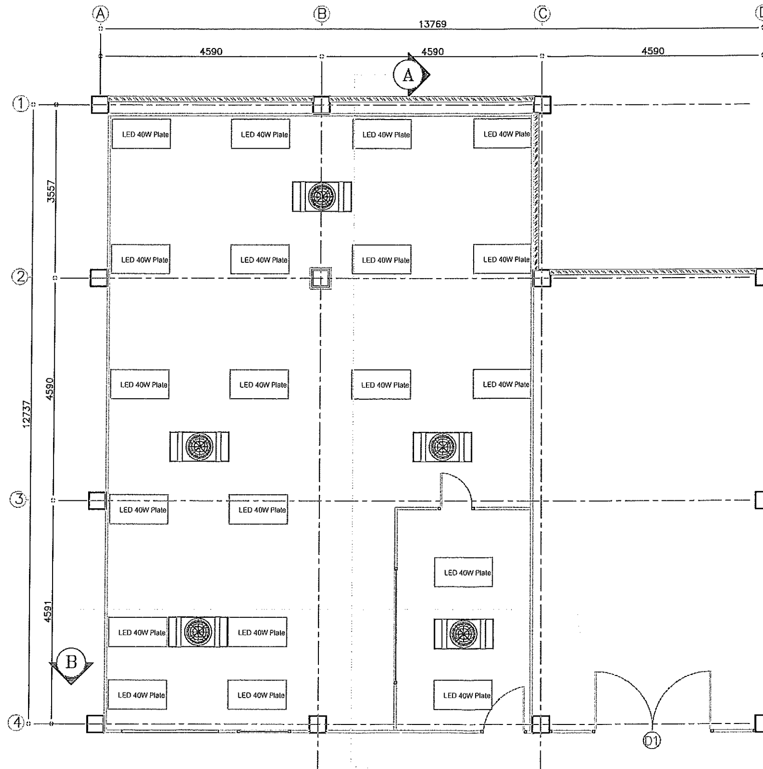
CEILING PLAN LAYOUT SCALE 1:75
