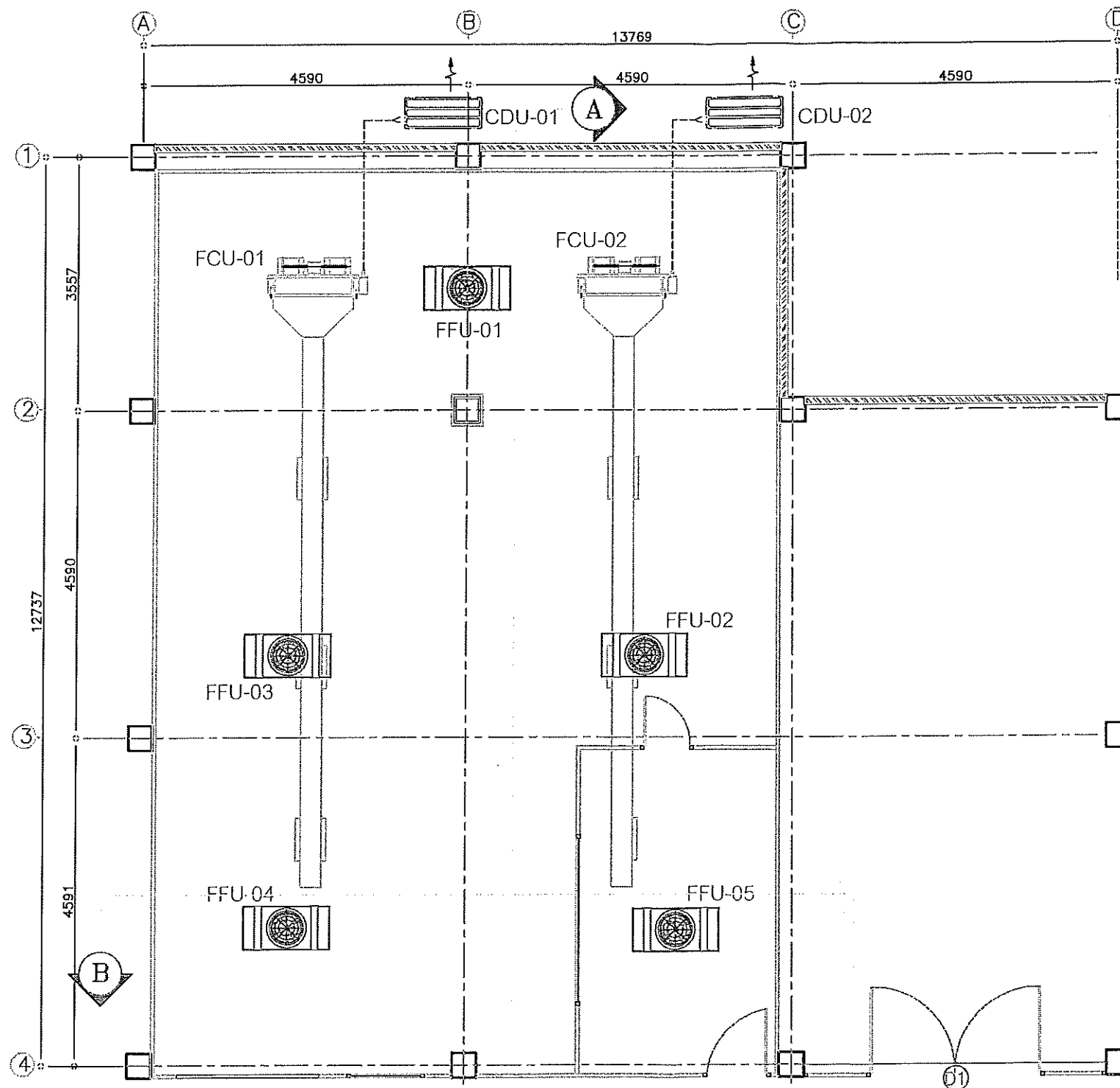
AIR CONDITION SYSTEM PLAN SCALE 1:75
