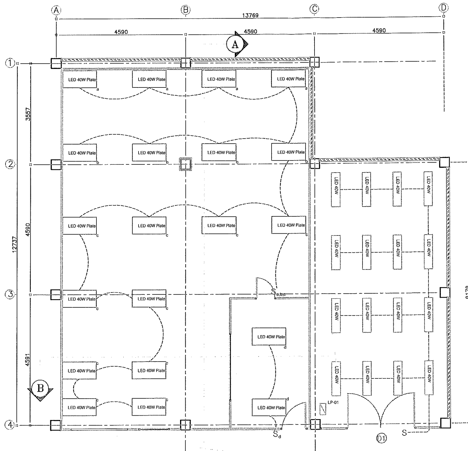
LIGHTING PLAN LAYOUT SCALE 1:75
