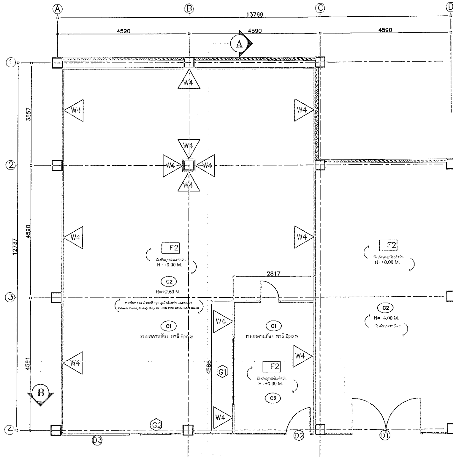
INTERIOR PLAN LAYOUT SCALE 1:75
