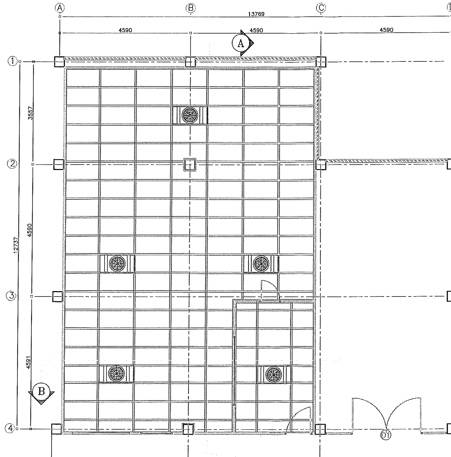
EXTRUDE CEILING GRID & FAN FILTER PLAN SCALE 1:75
